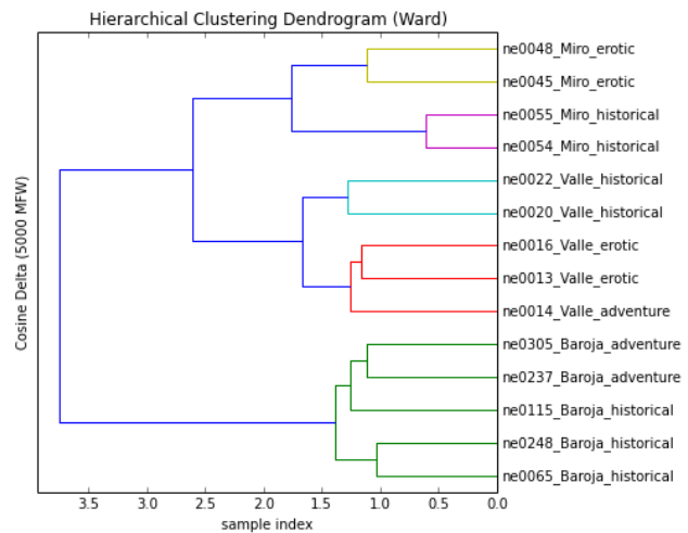
Figure 1: Dendrogram from Cosine Delta
